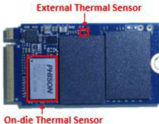
Figure 2-1 Thermal Sensor
